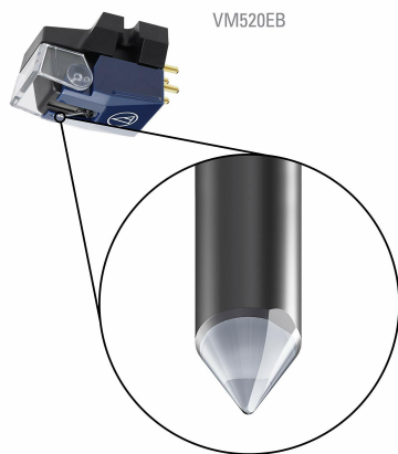
Stylus Shape: Elliptical Stylus Construction: Bonded Round Shank
