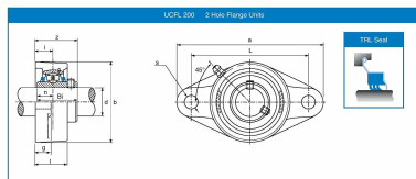
UCFL 200 2 Hole Flange Units (Normal Duty)
