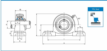
UCPX 00 Pillow Block (Medium Duty)
